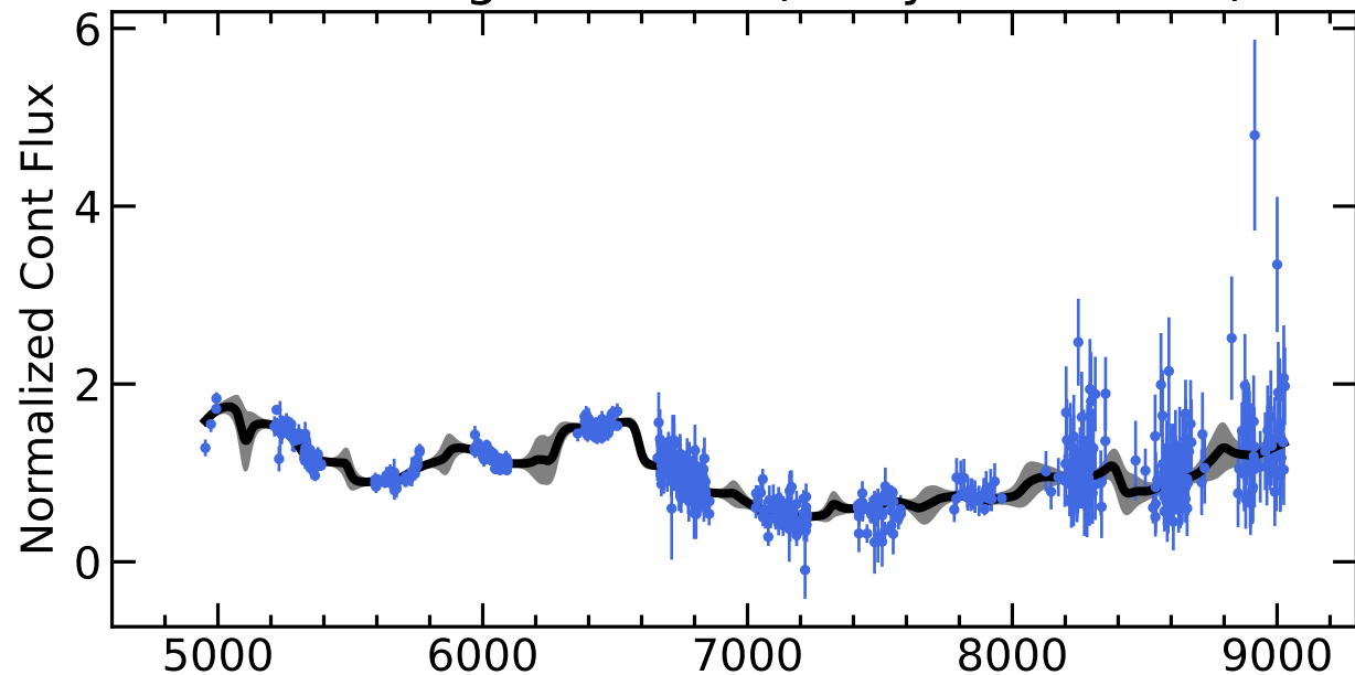
RM344 Light Curves (w/ PyROA model)
