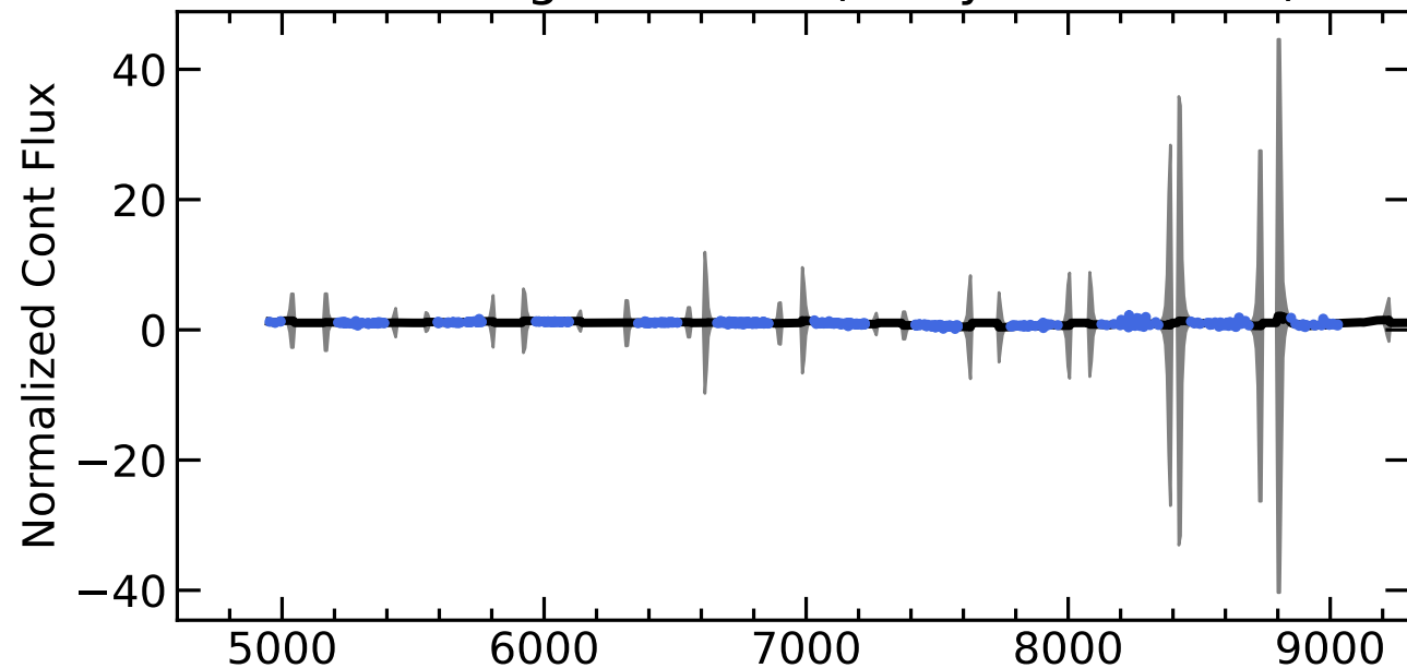
RM345 Light Curves (w/ PyROA model)
