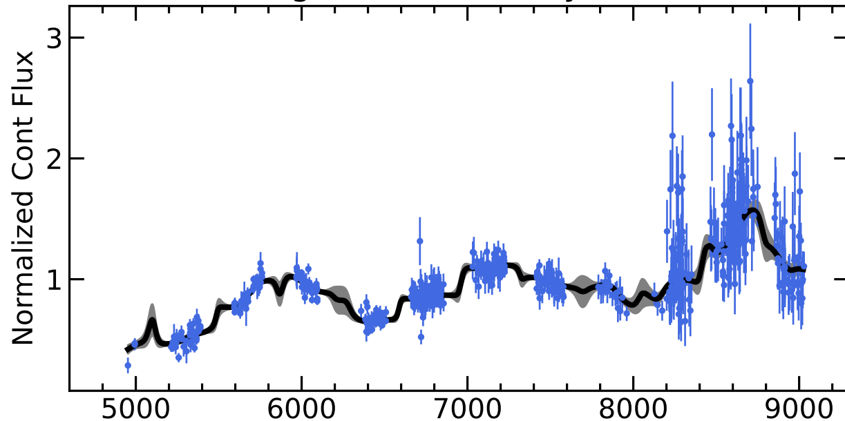
RM346 Light Curves (w/ PyROA model)
