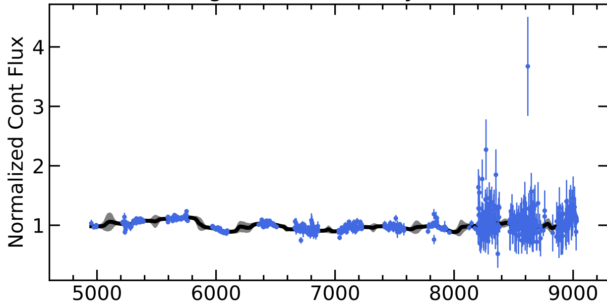
RM348 Light Curves (w/ PyROA model)
