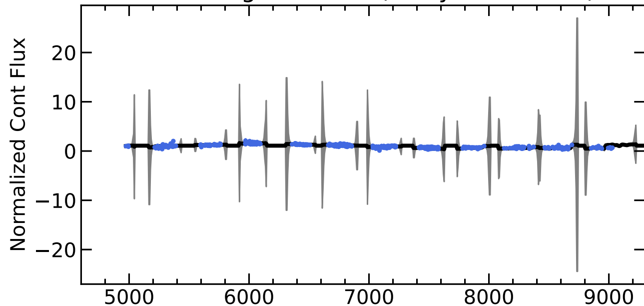
RM349 Light Curves (w/ PyROA model)
