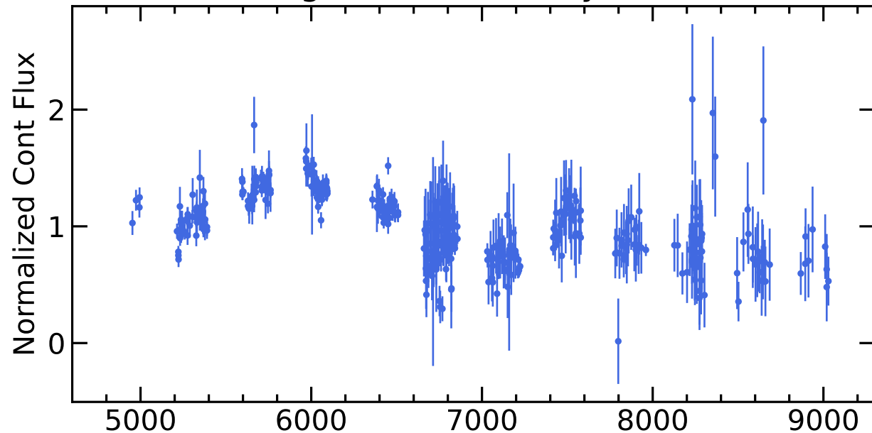
RM351 Light Curves (w/ PyROA model)
