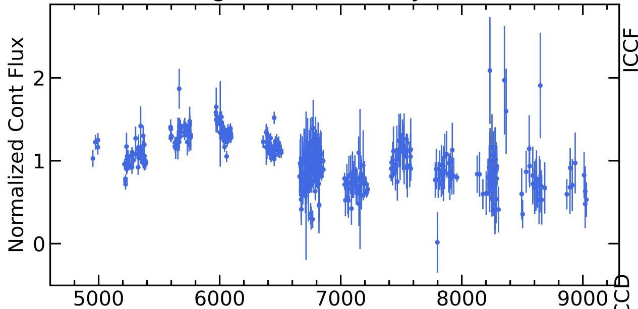
RM351 Light Curves (w/ PyROA model)
