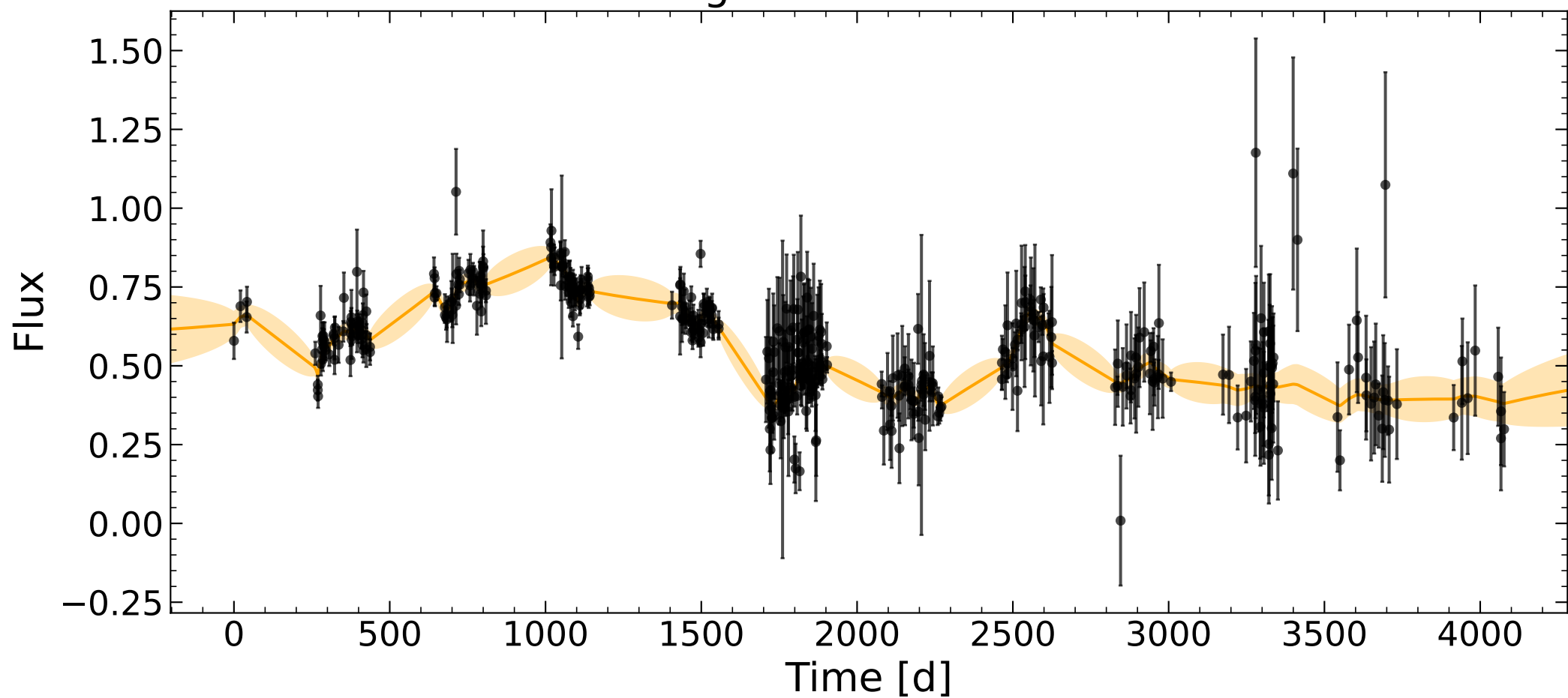
Light Curve of cont
