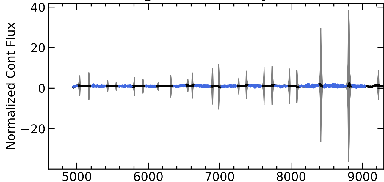
RM352 Light Curves (w/ PyROA model)
