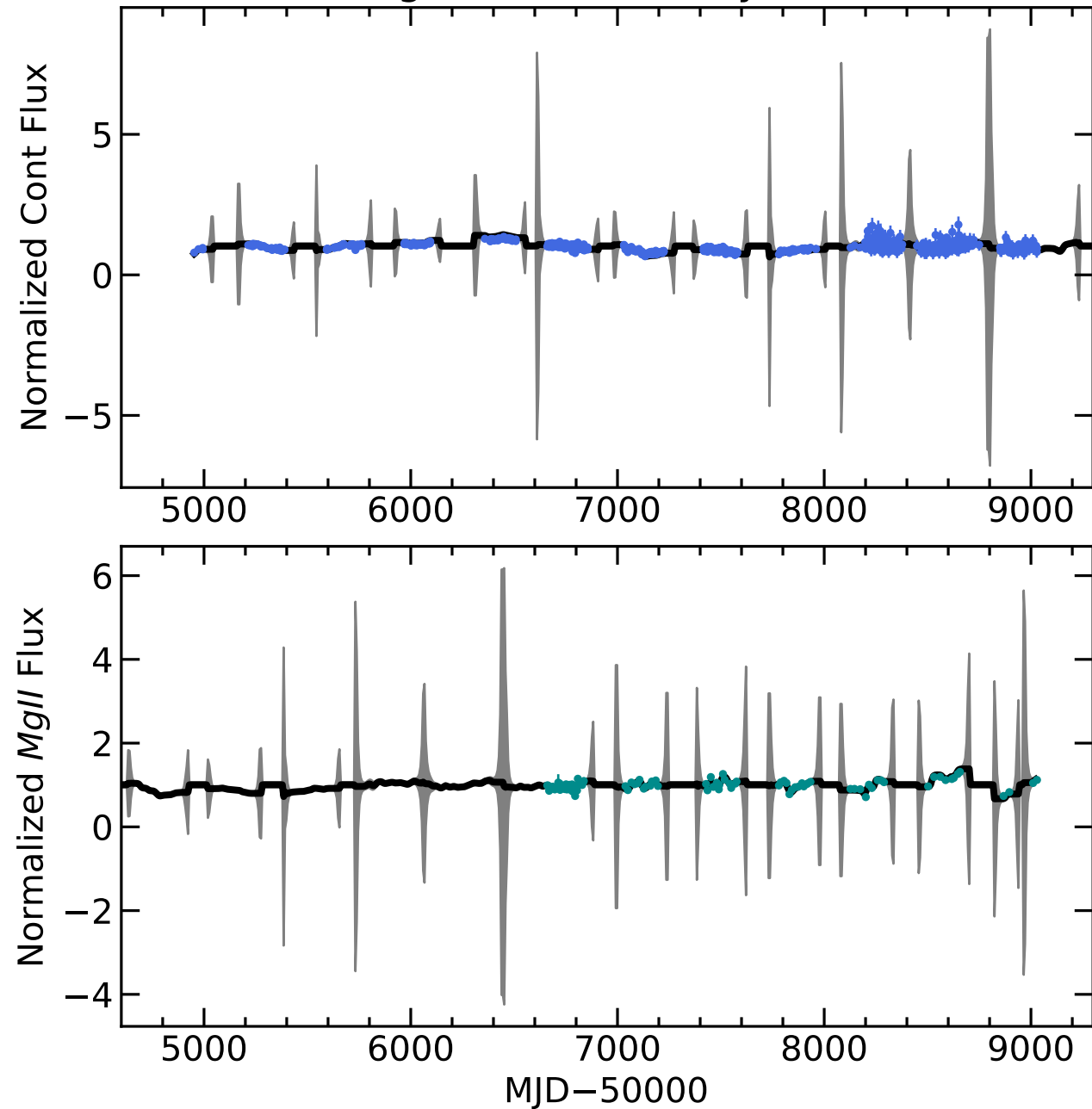
RM353 Light Curves (w/ PyROA model)
