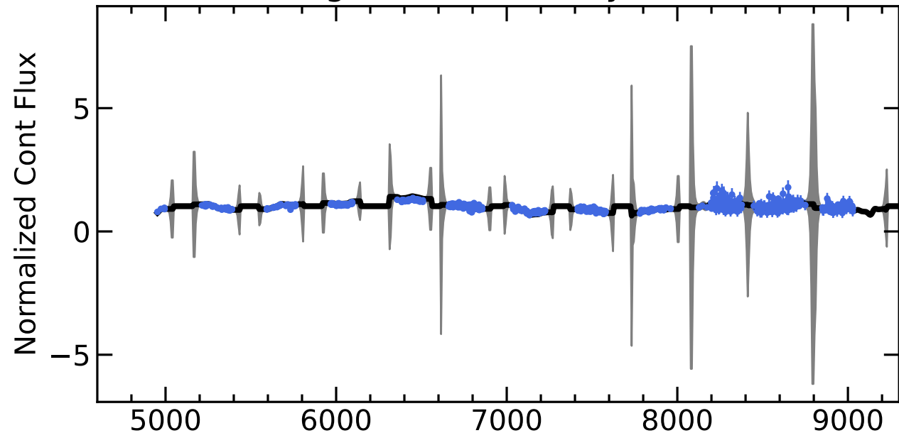
RM353 Light Curves (w/ PyROA model)
