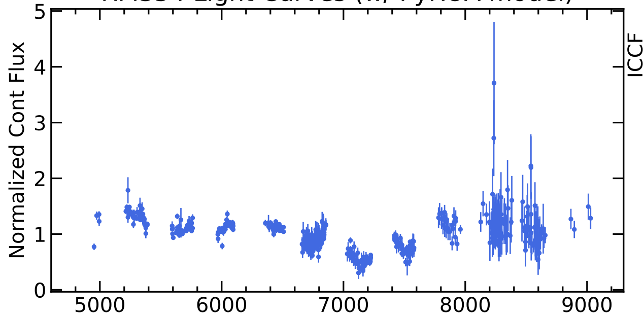
RM354 Light Curves (w/ PyROA model)
