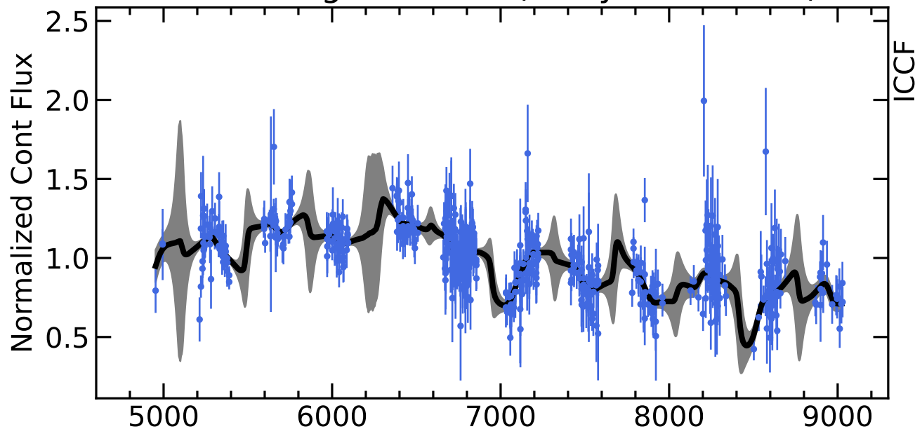
RM355 Light Curves (w/ PyROA model)
