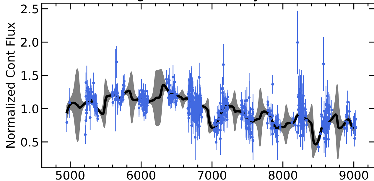
RM355 Light Curves (w/ PyROA model)
