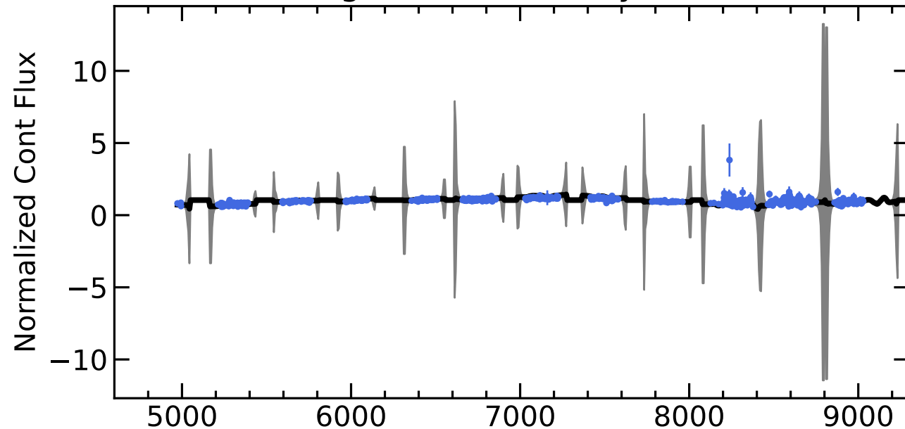
RM357 Light Curves (w/ PyROA model)
