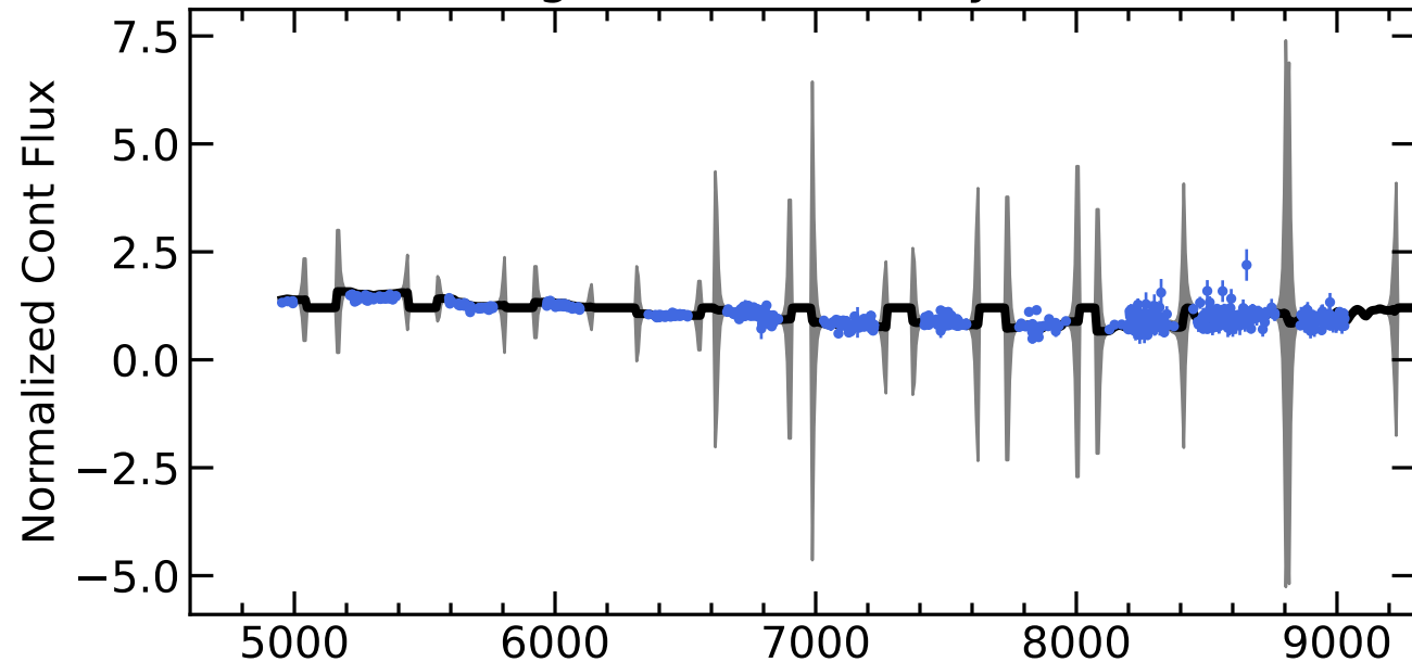
RM359 Light Curves (w/ PyROA model)
