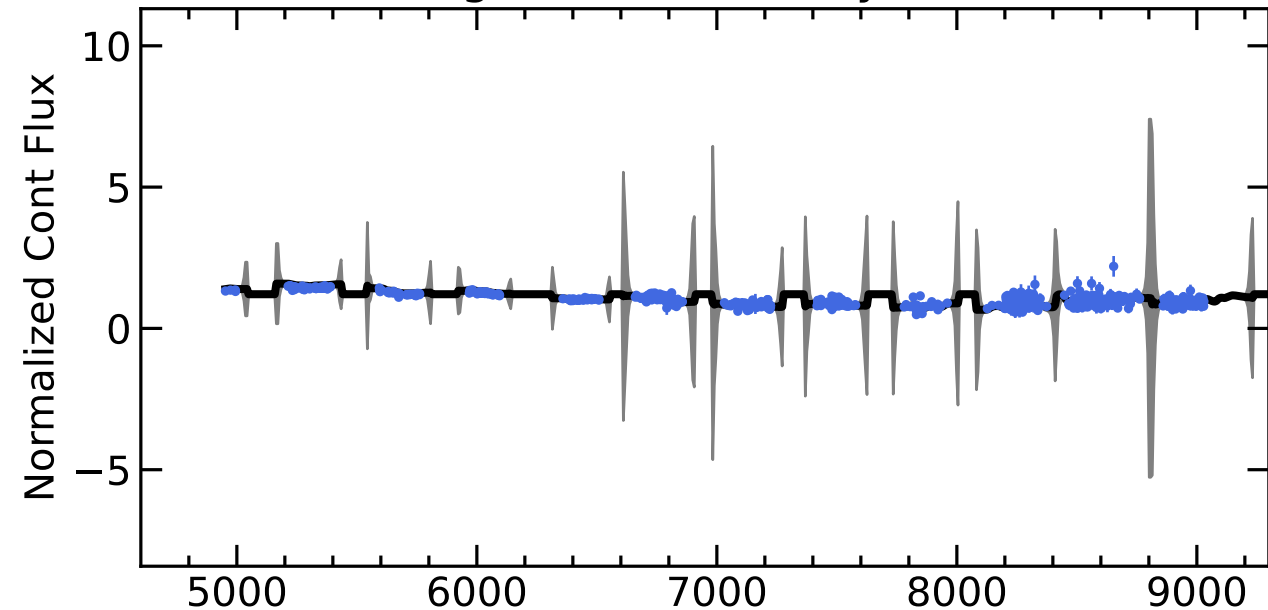
RM359 Light Curves (w/ PyROA model)
