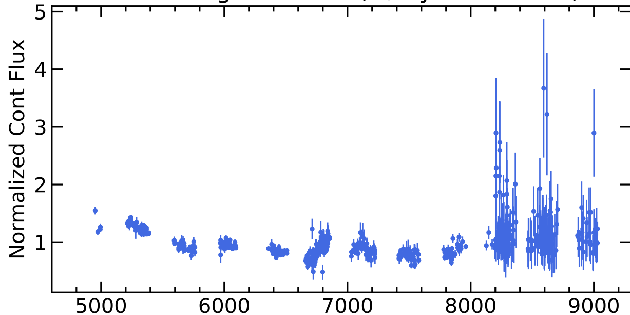
RM360 Light Curves (w/ PyROA model)
