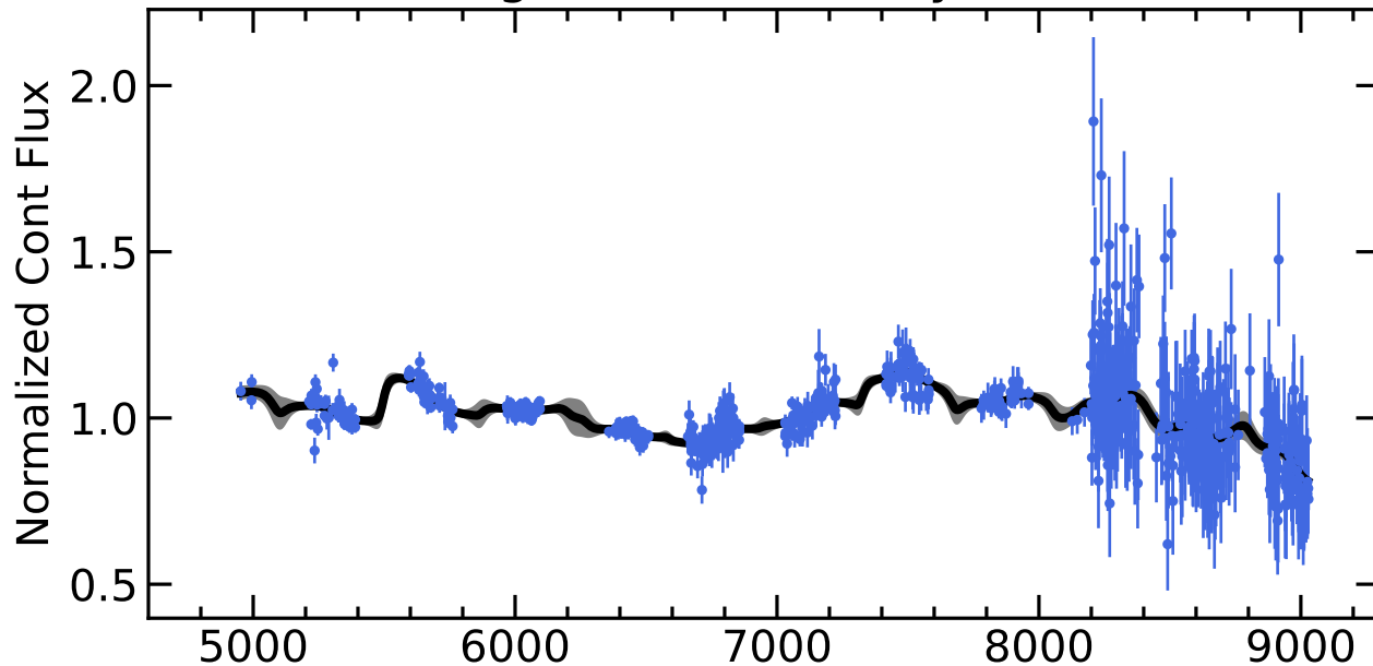
RM361 Light Curves (w/ PyROA model)
