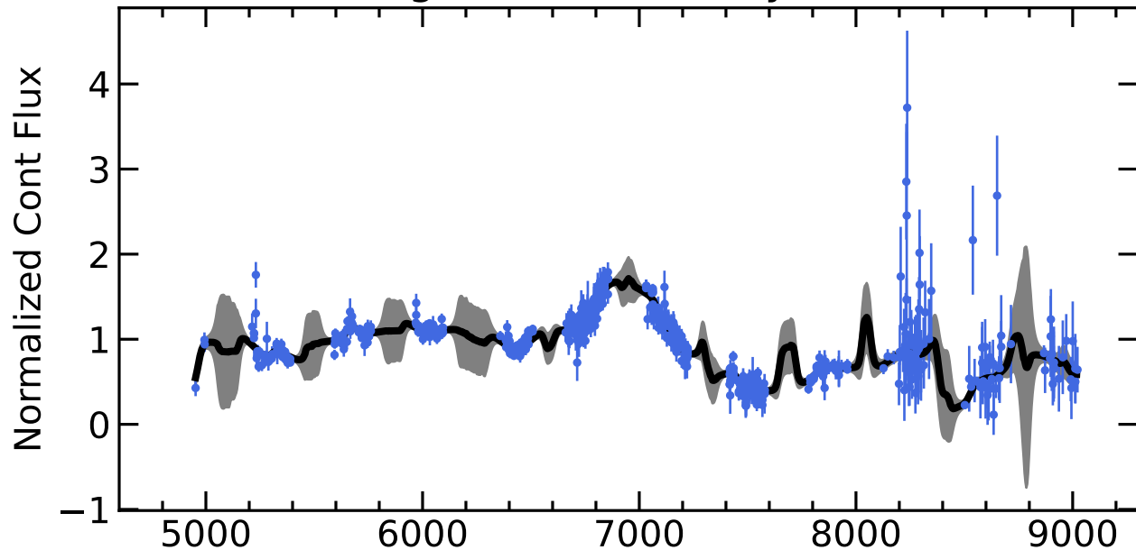
RM362 Light Curves (w/ PyROA model)
