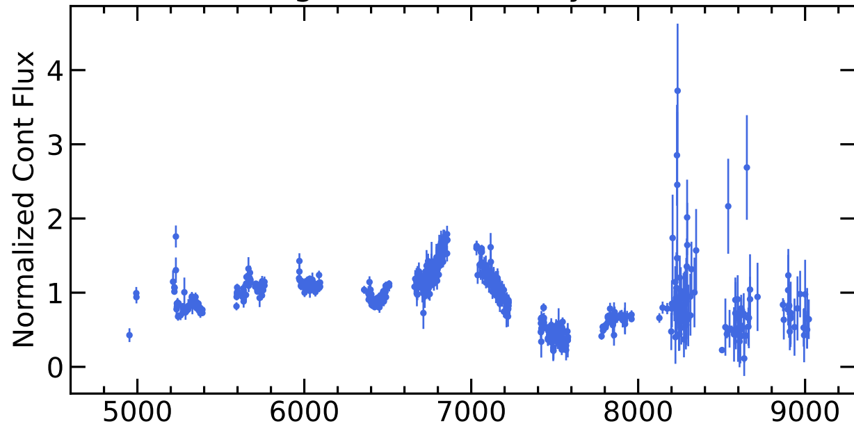
RM362 Light Curves (w/ PyROA model)
