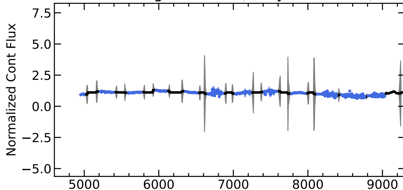
RM363 Light Curves (w/ PyROA model)
