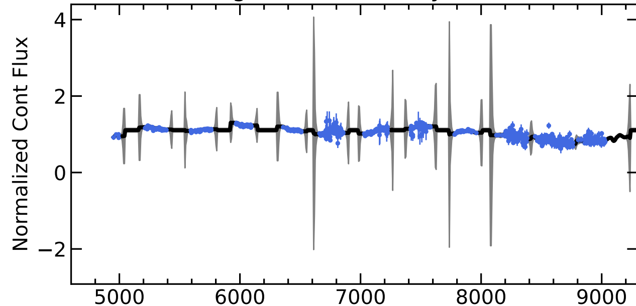
RM363 Light Curves (w/ PyROA model)
