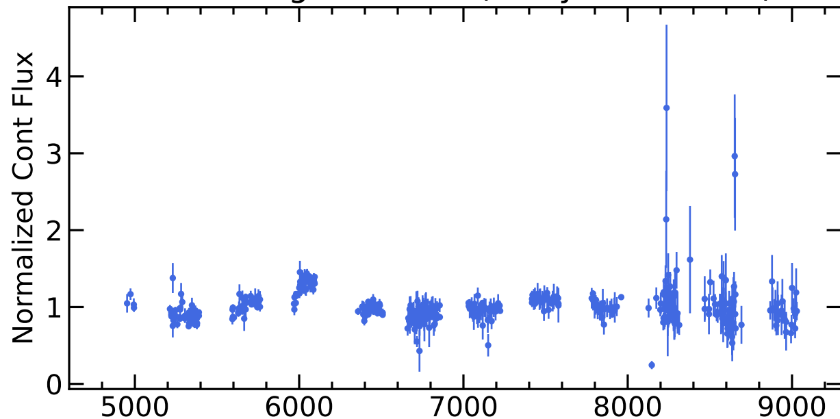
RM364 Light Curves (w/ PyROA model)
