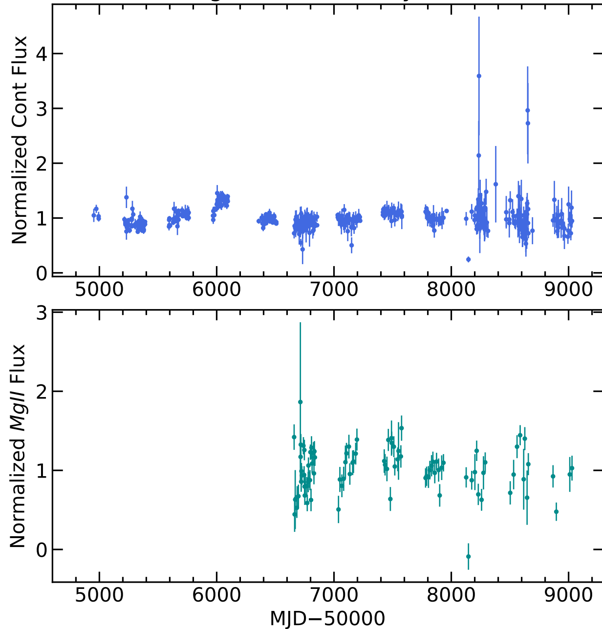
RM364 Light Curves (w/ PyROA model)
