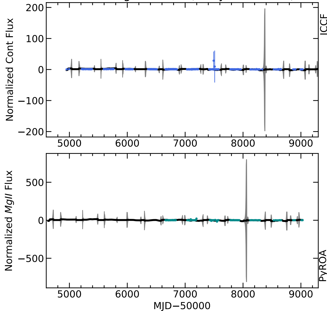
RM365 Light Curves (w/ PyROA model)
