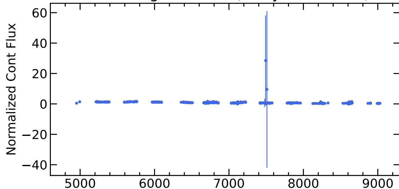
RM365 Light Curves (w/ PyROA model)
