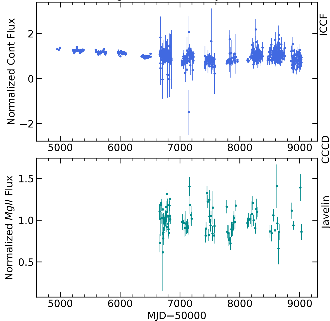
RM366 Light Curves (w/ PyROA model)
