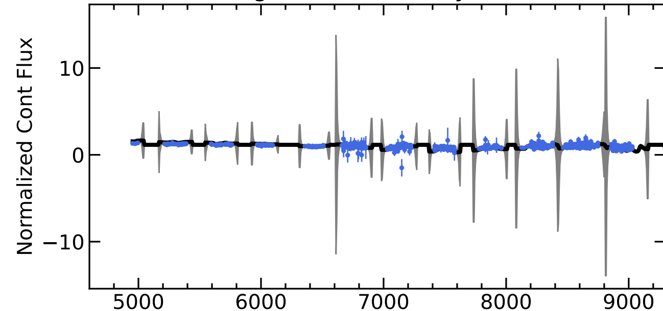
RM366 Light Curves (w/ PyROA model)
