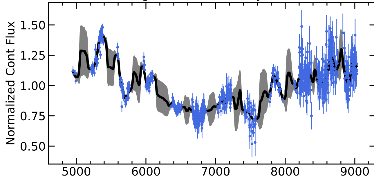
RM369 Light Curves (w/ PyROA model)
