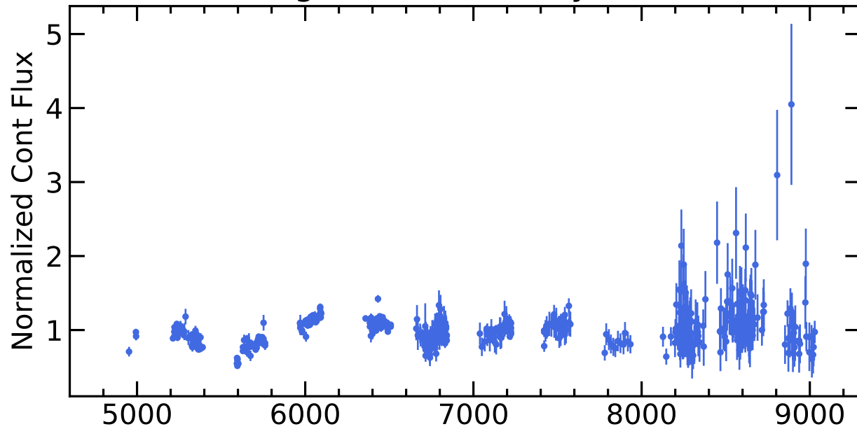
RM370 Light Curves (w/ PyROA model)
