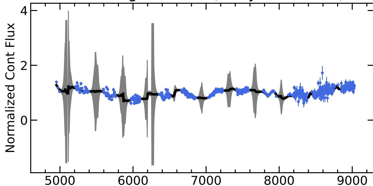
RM371 Light Curves (w/ PyROA model)
