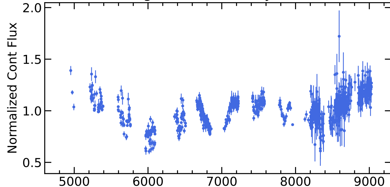
RM371 Light Curves (w/ PyROA model)
