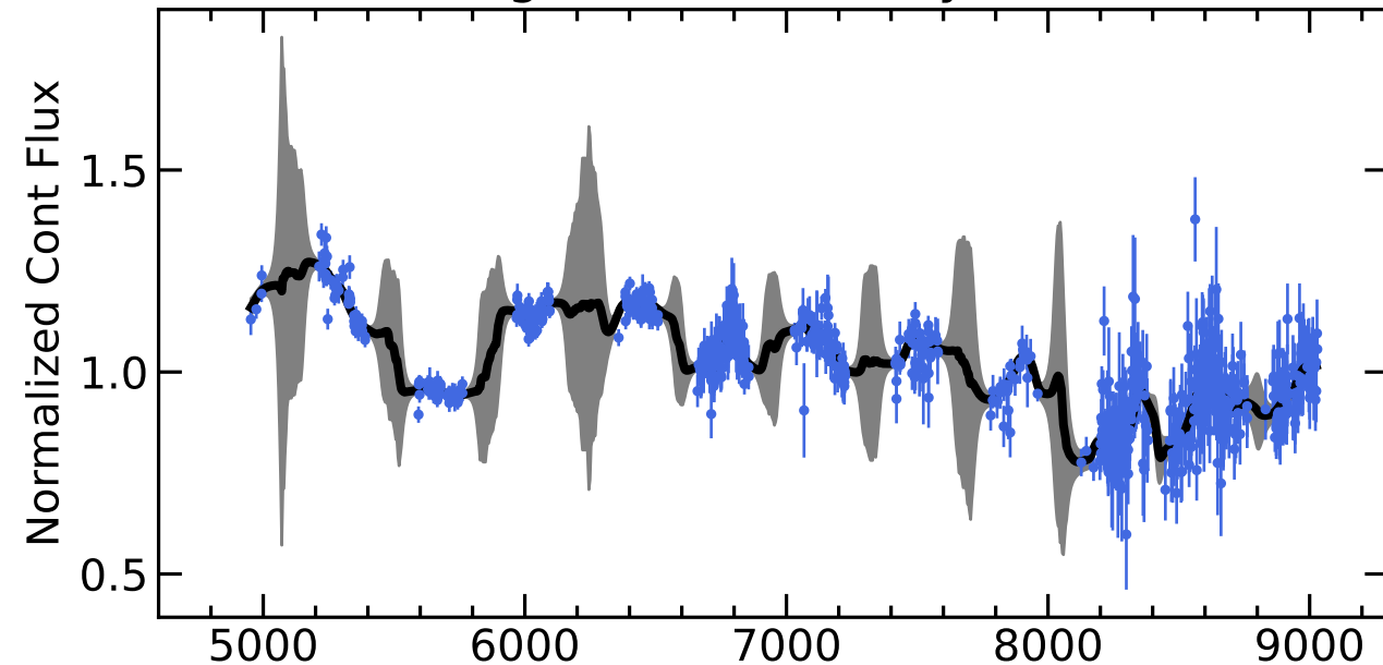
RM373 Light Curves (w/ PyROA model)
