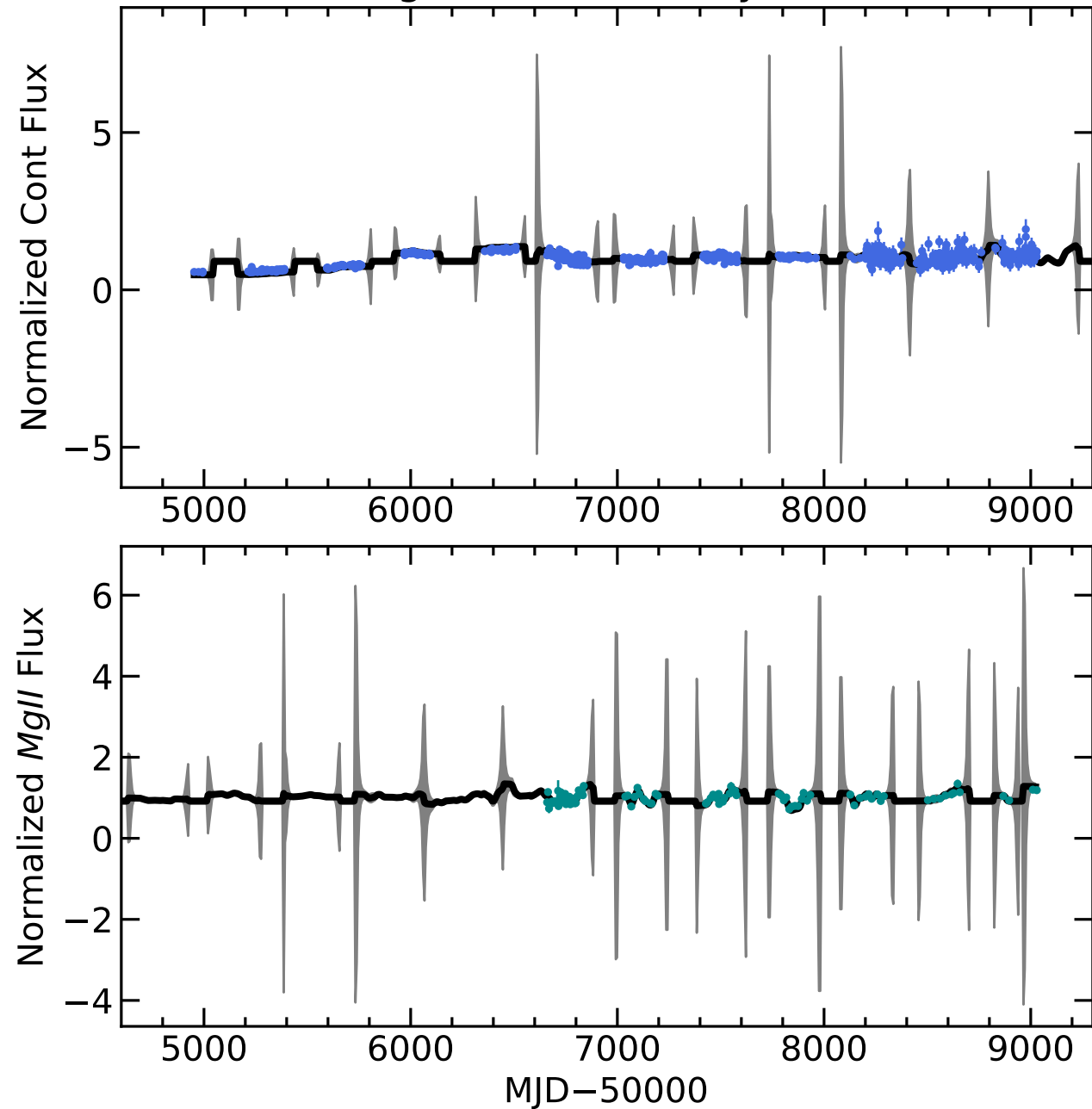
RM374 Light Curves (w/ PyROA model)
