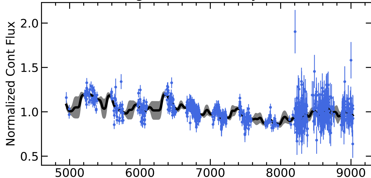
RM377 Light Curves (w/ PyROA model)
