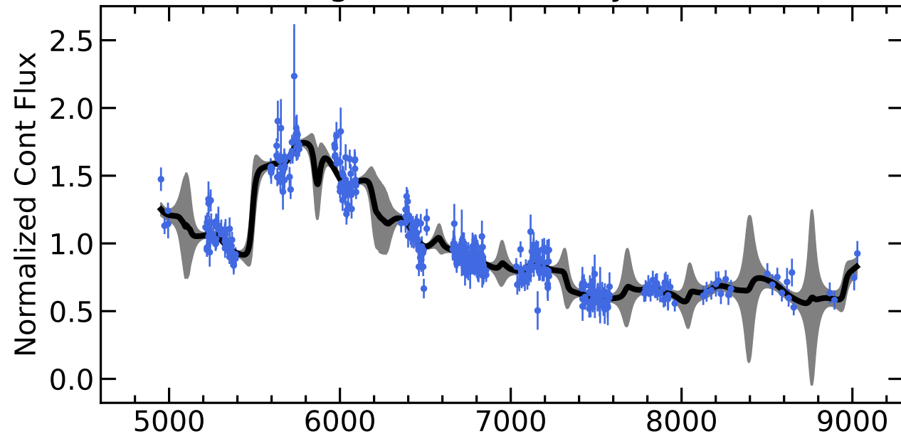
RM378 Light Curves (w/ PyROA model)
