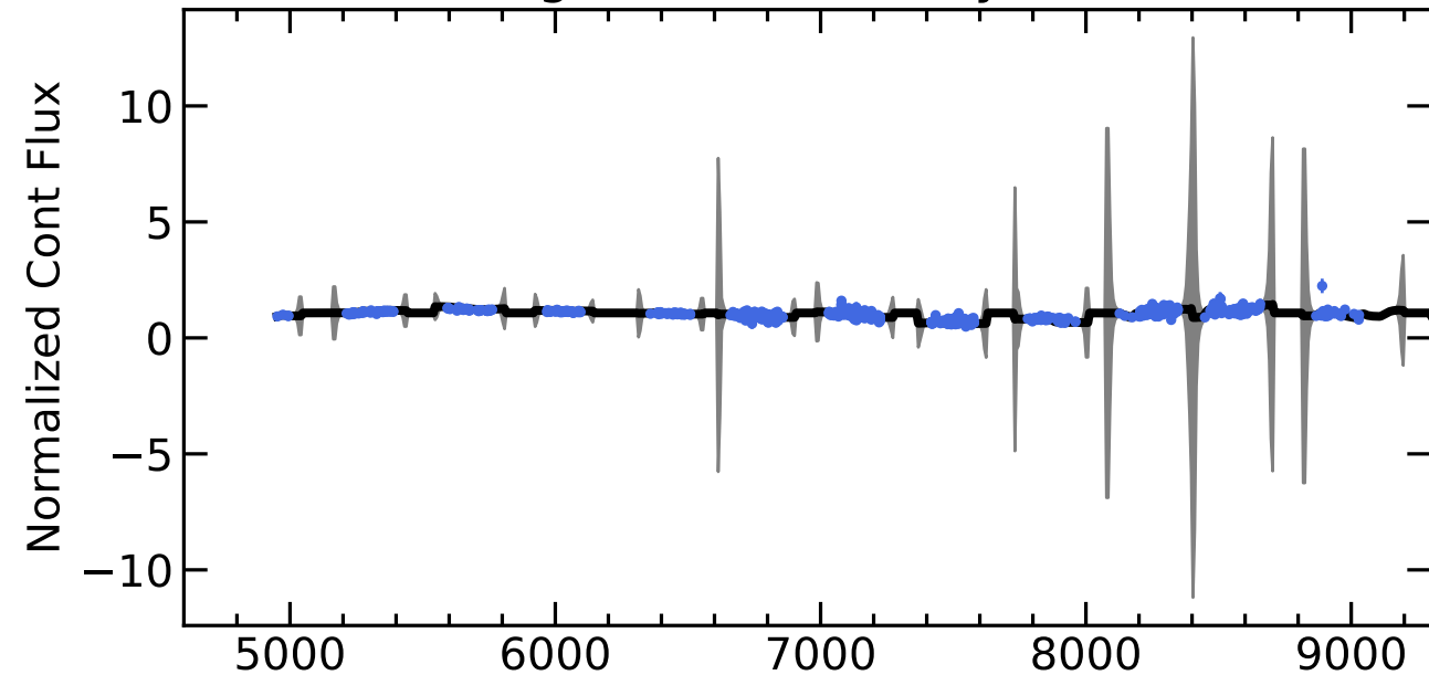
RM379 Light Curves (w/ PyROA model)
