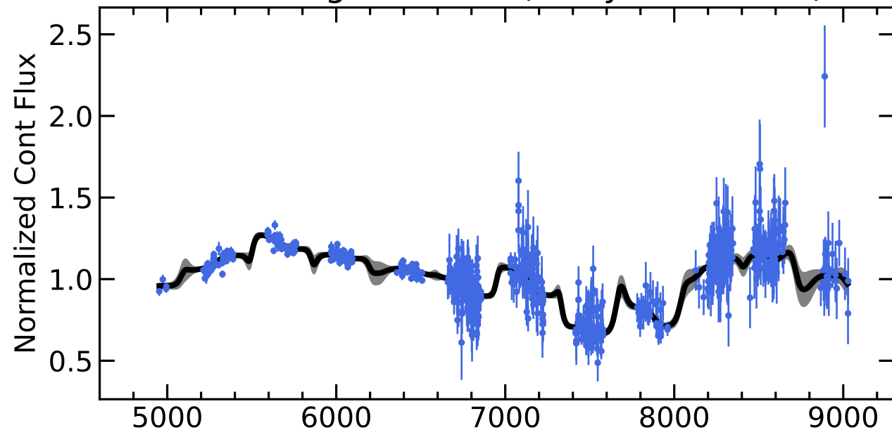
RM379 Light Curves (w/ PyROA model)
