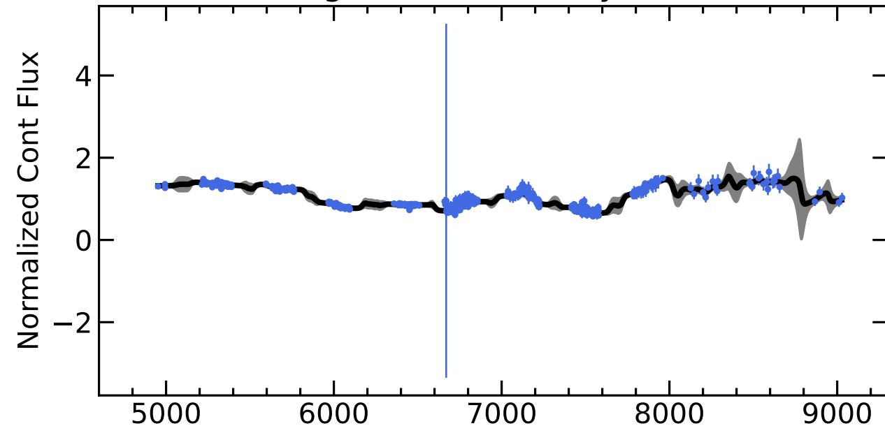
RM380 Light Curves (w/ PyROA model)
