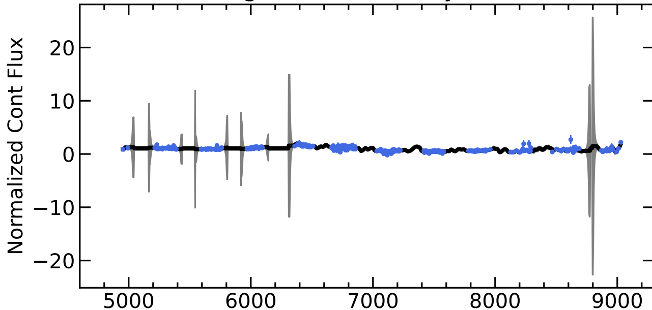
RM382 Light Curves (w/ PyROA model)
