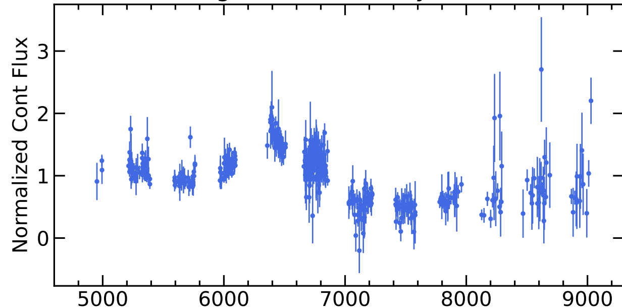
RM382 Light Curves (w/ PyROA model)
