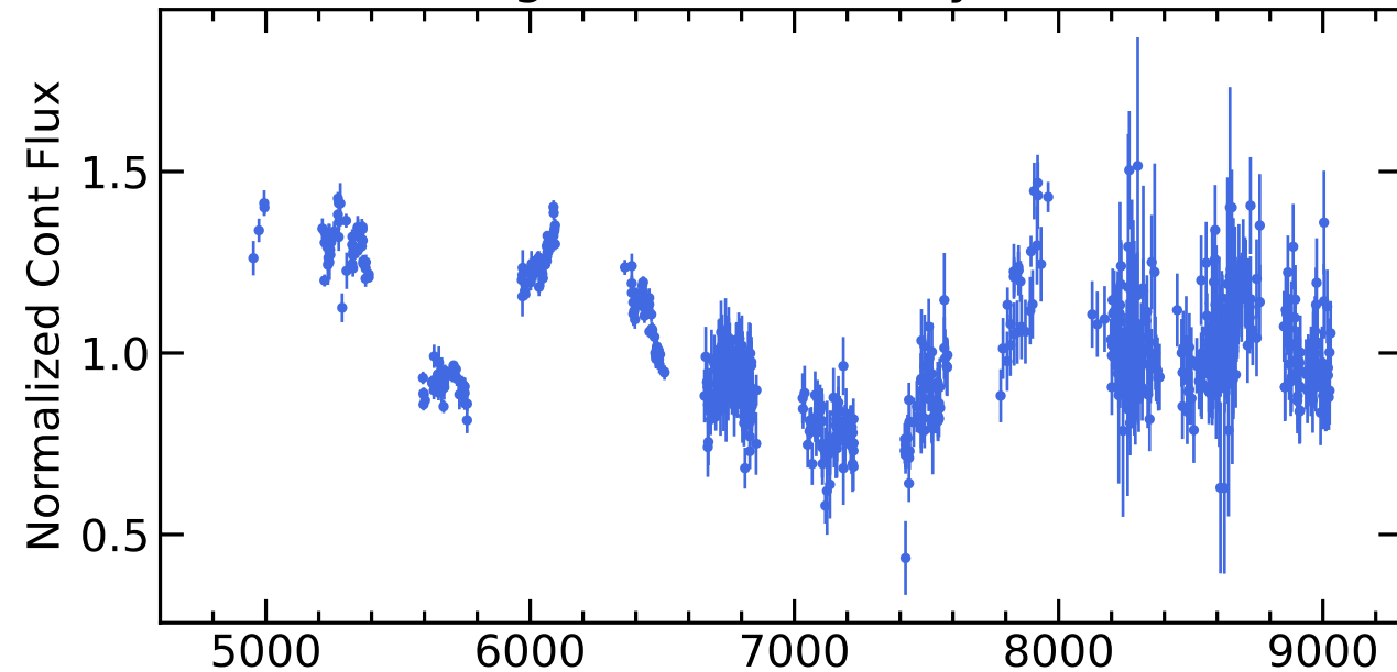
RM384 Light Curves (w/ PyROA model)
