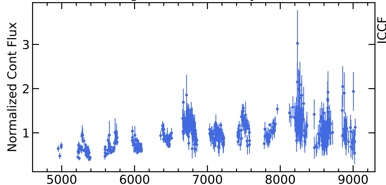
RM385 Light Curves (w/ PyROA model)
