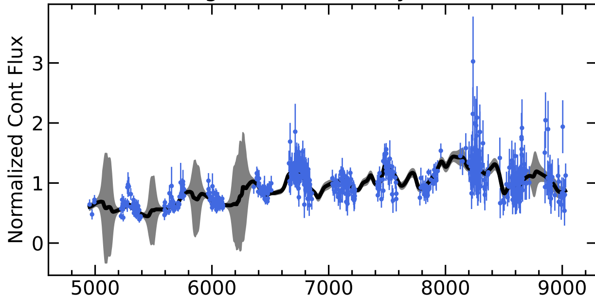
RM385 Light Curves (w/ PyROA model)
