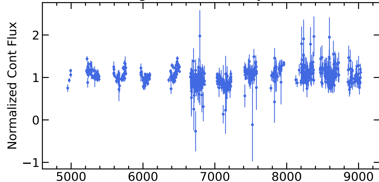
RM386 Light Curves (w/ PyROA model)
