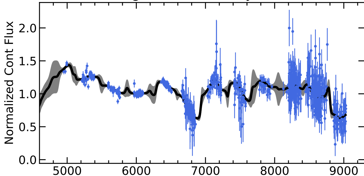
RM387 Light Curves (w/ PyROA model)
