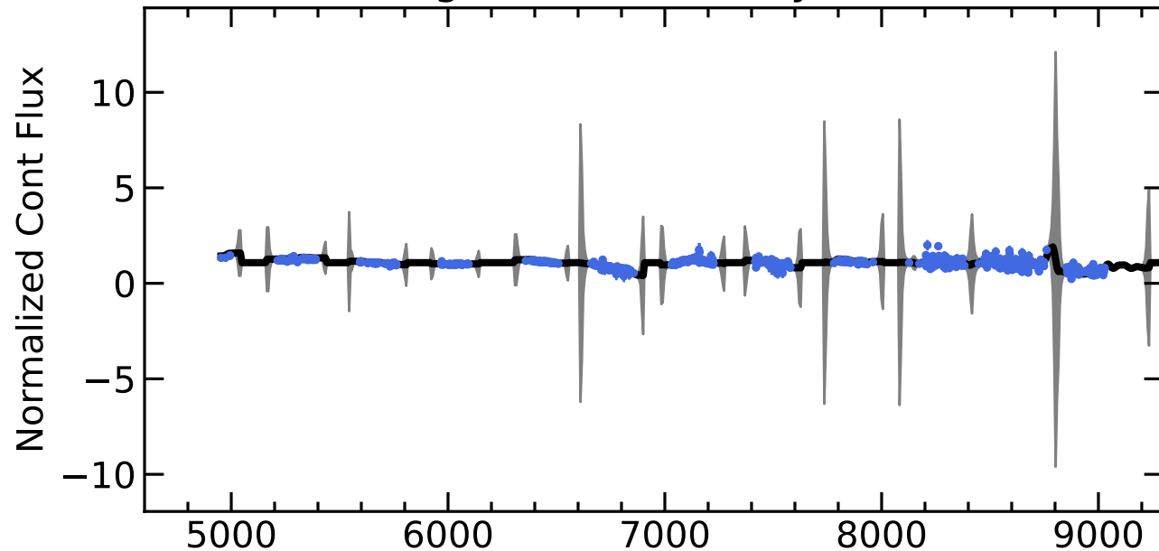
RM387 Light Curves (w/ PyROA model)
