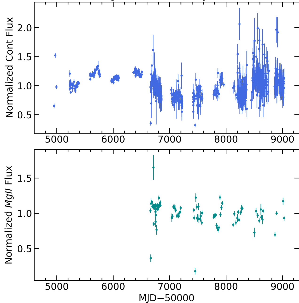
RM389 Light Curves (w/ PyROA model)
