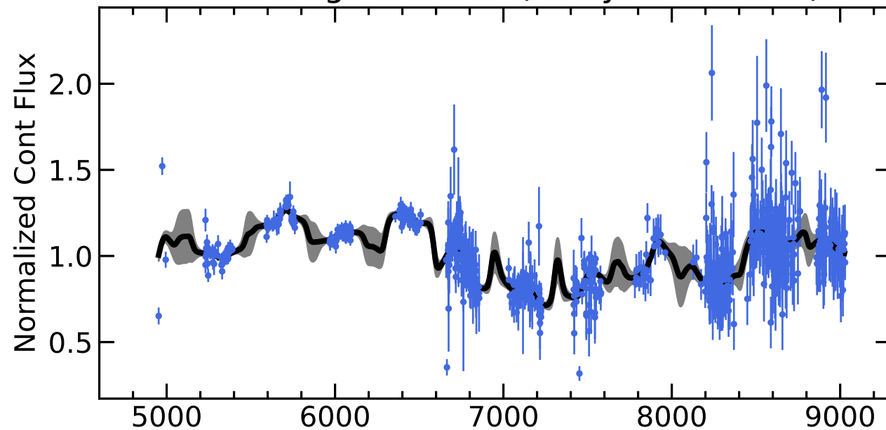
RM389 Light Curves (w/ PyROA model)
