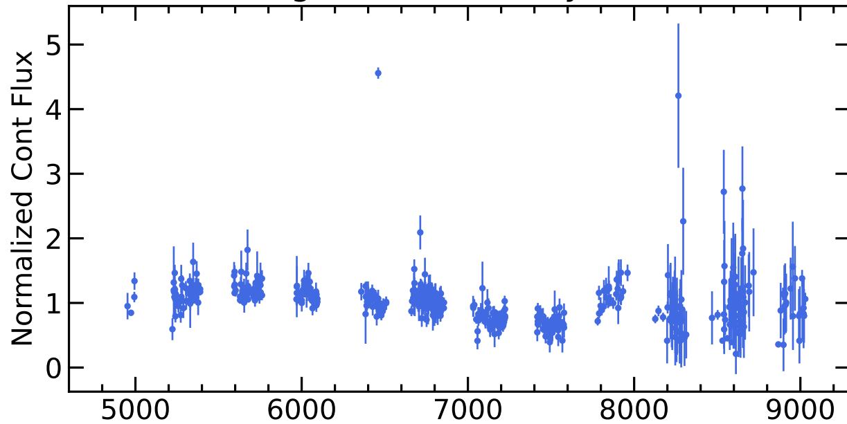
RM390 Light Curves (w/ PyROA model)
