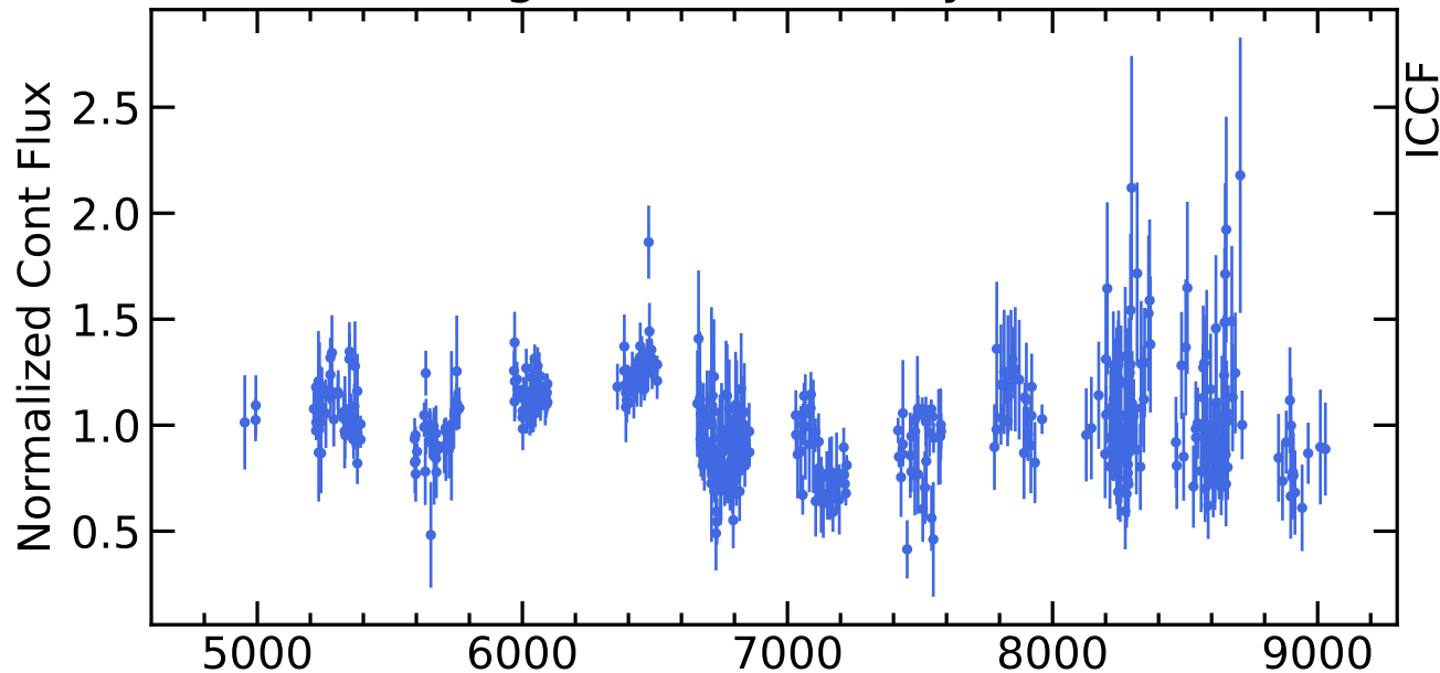
RM391 Light Curves (w/ PyROA model)
