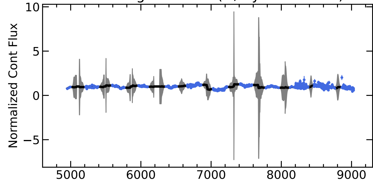
RM392 Light Curves (w/ PyROA model)
