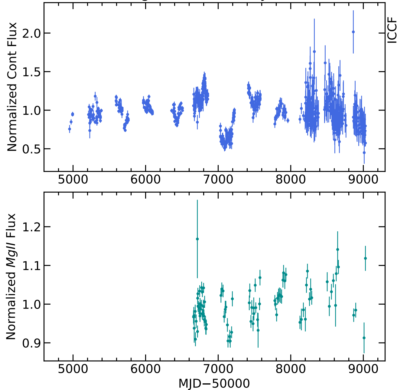
RM392 Light Curves (w/ PyROA model)
