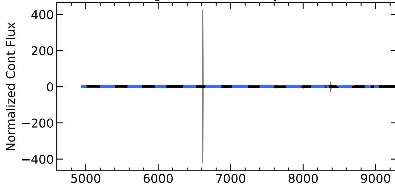
RM394 Light Curves (w/ PyROA model)
