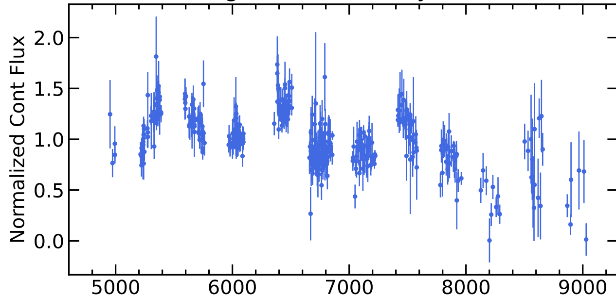
RM395 Light Curves (w/ PyROA model)
