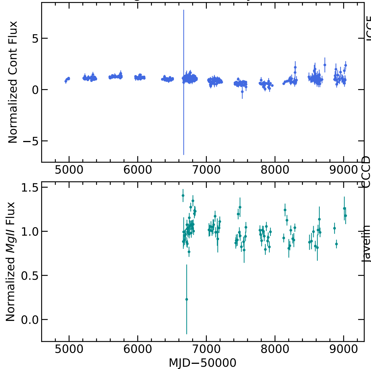
RM396 Light Curves (w/ PyROA model)
