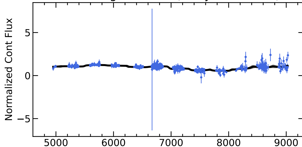
RM396 Light Curves (w/ PyROA model)
