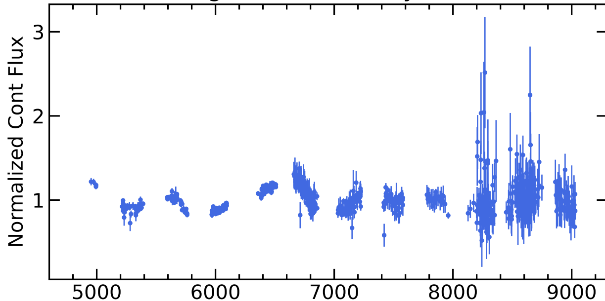
RM398 Light Curves (w/ PyROA model)
