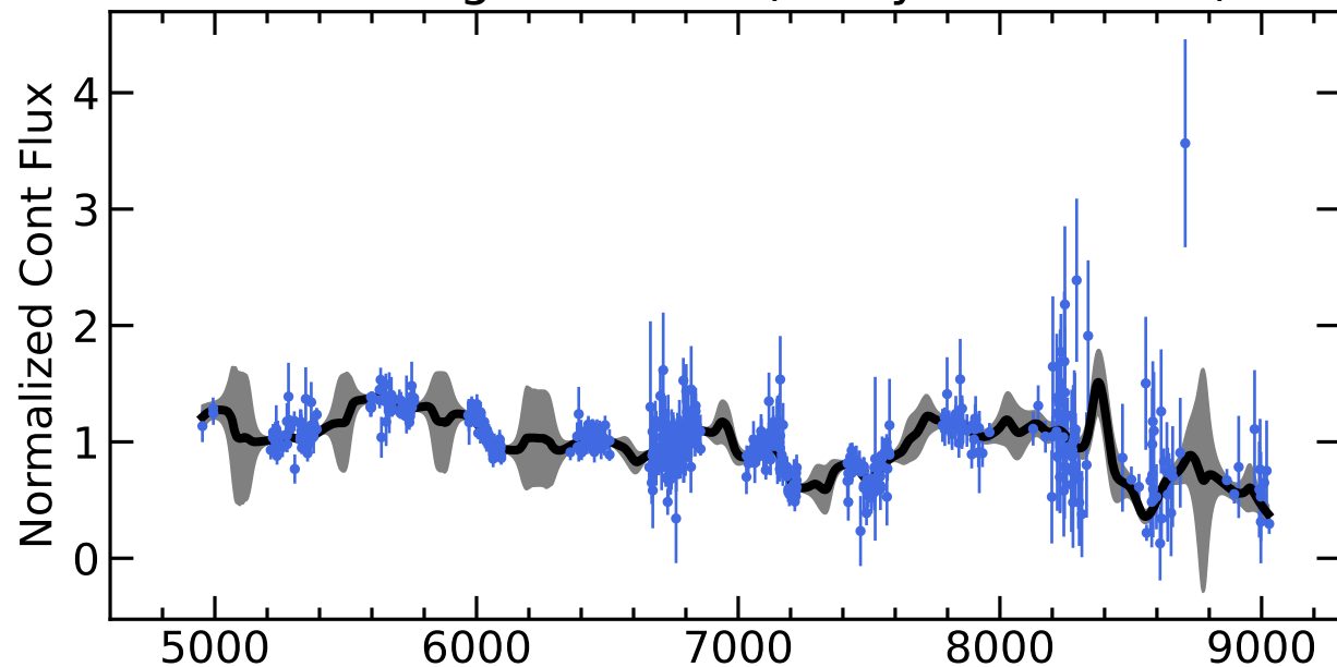
RM400 Light Curves (w/ PyROA model)
