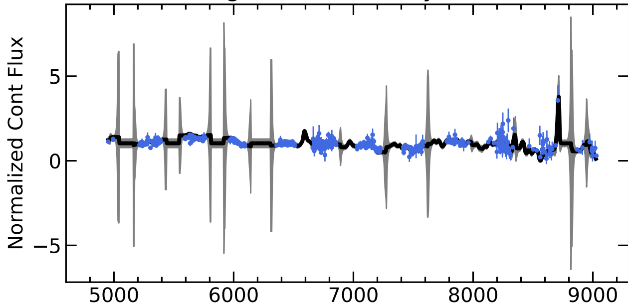
RM400 Light Curves (w/ PyROA model)
