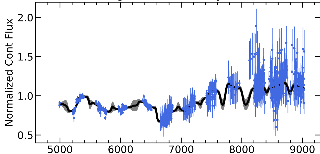
RM401 Light Curves (w/ PyROA model)
