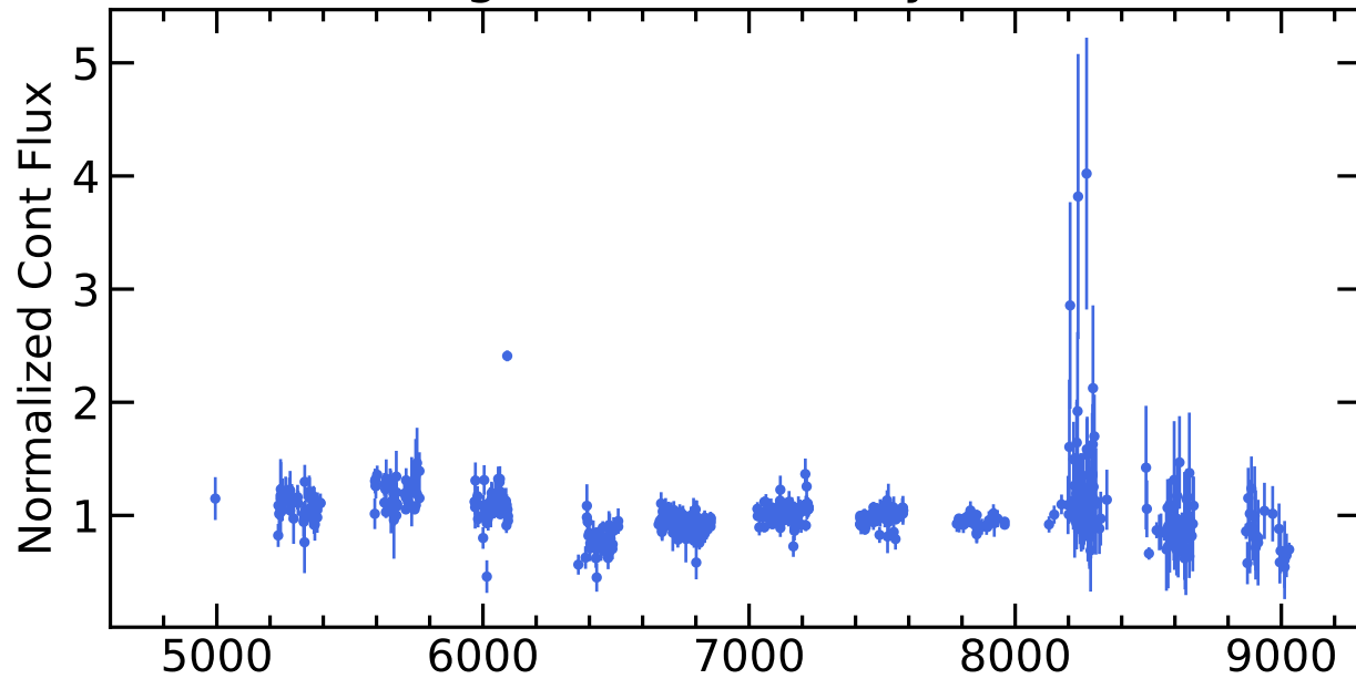
RM402 Light Curves (w/ PyROA model)
