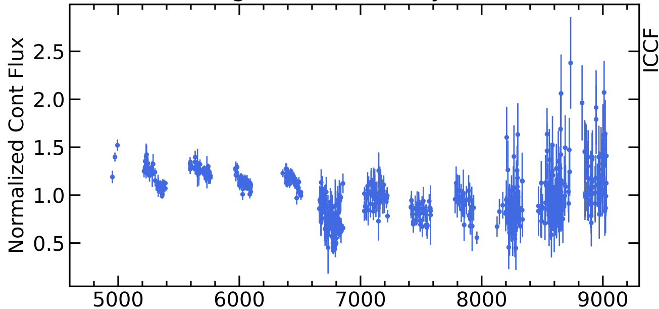
RM403 Light Curves (w/ PyROA model)
