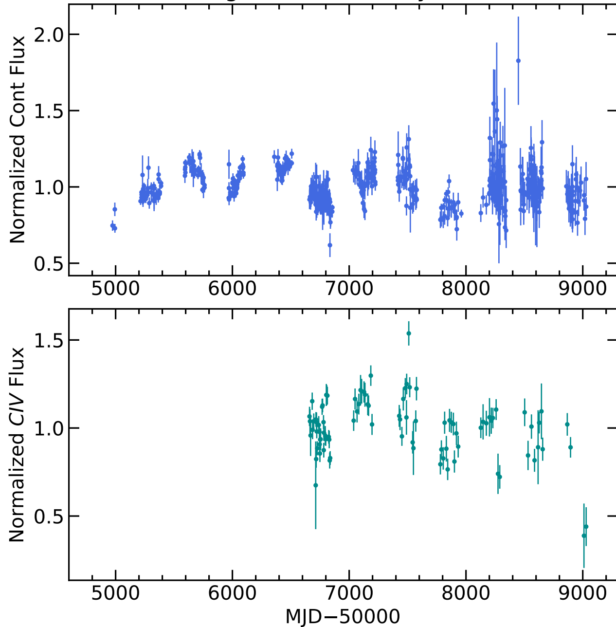
RM404 Light Curves (w/ PyROA model)
