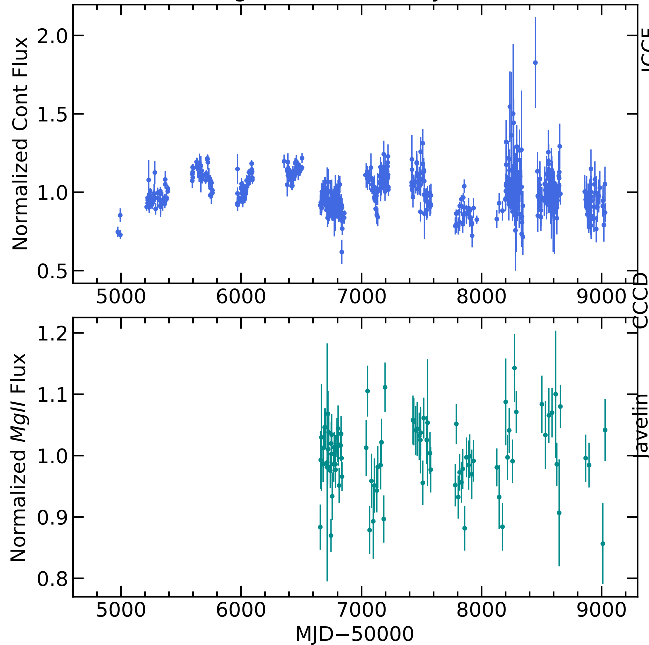
RM404 Light Curves (w/ PyROA model)
