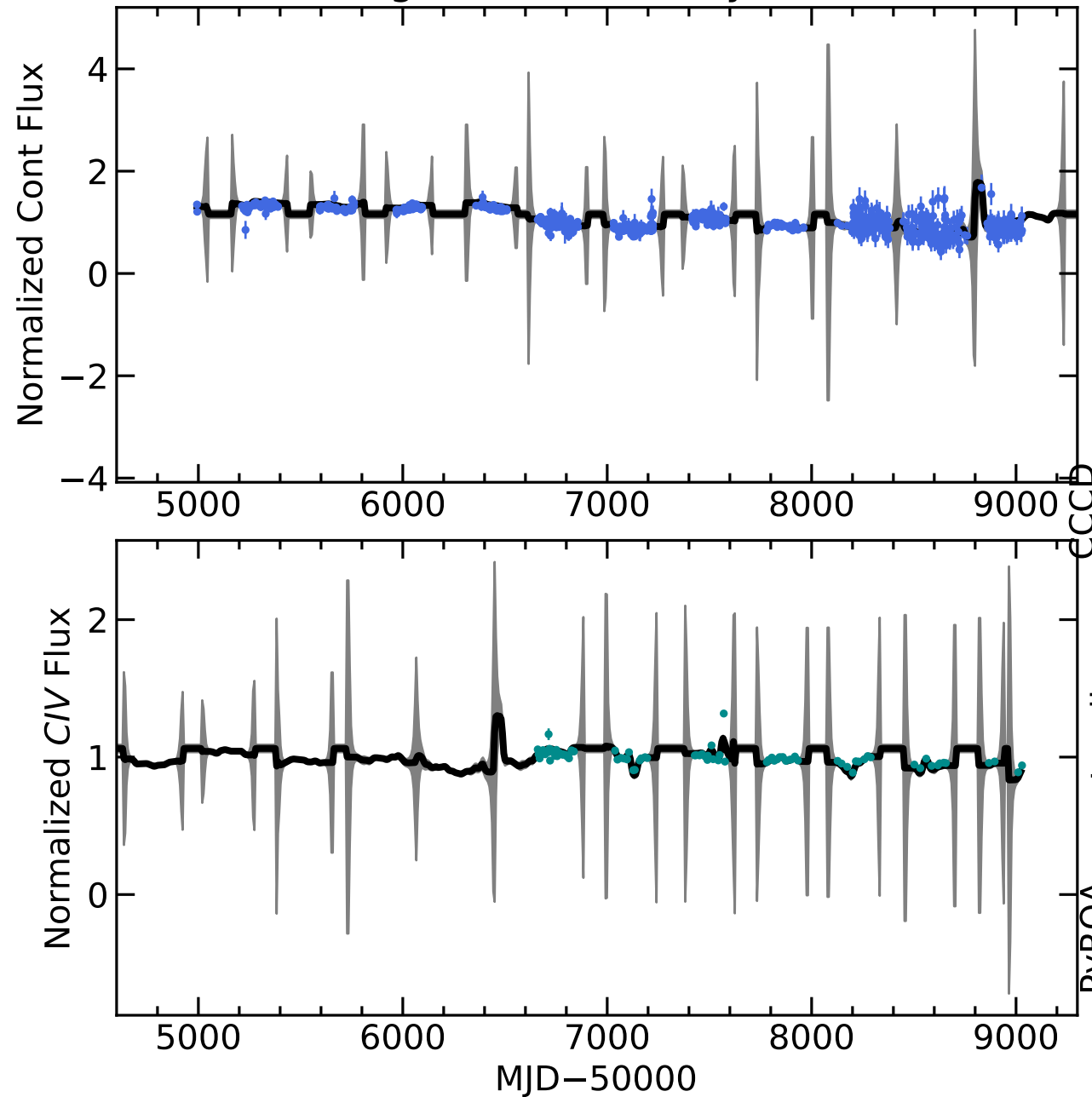
RM405 Light Curves (w/ PyROA model)
