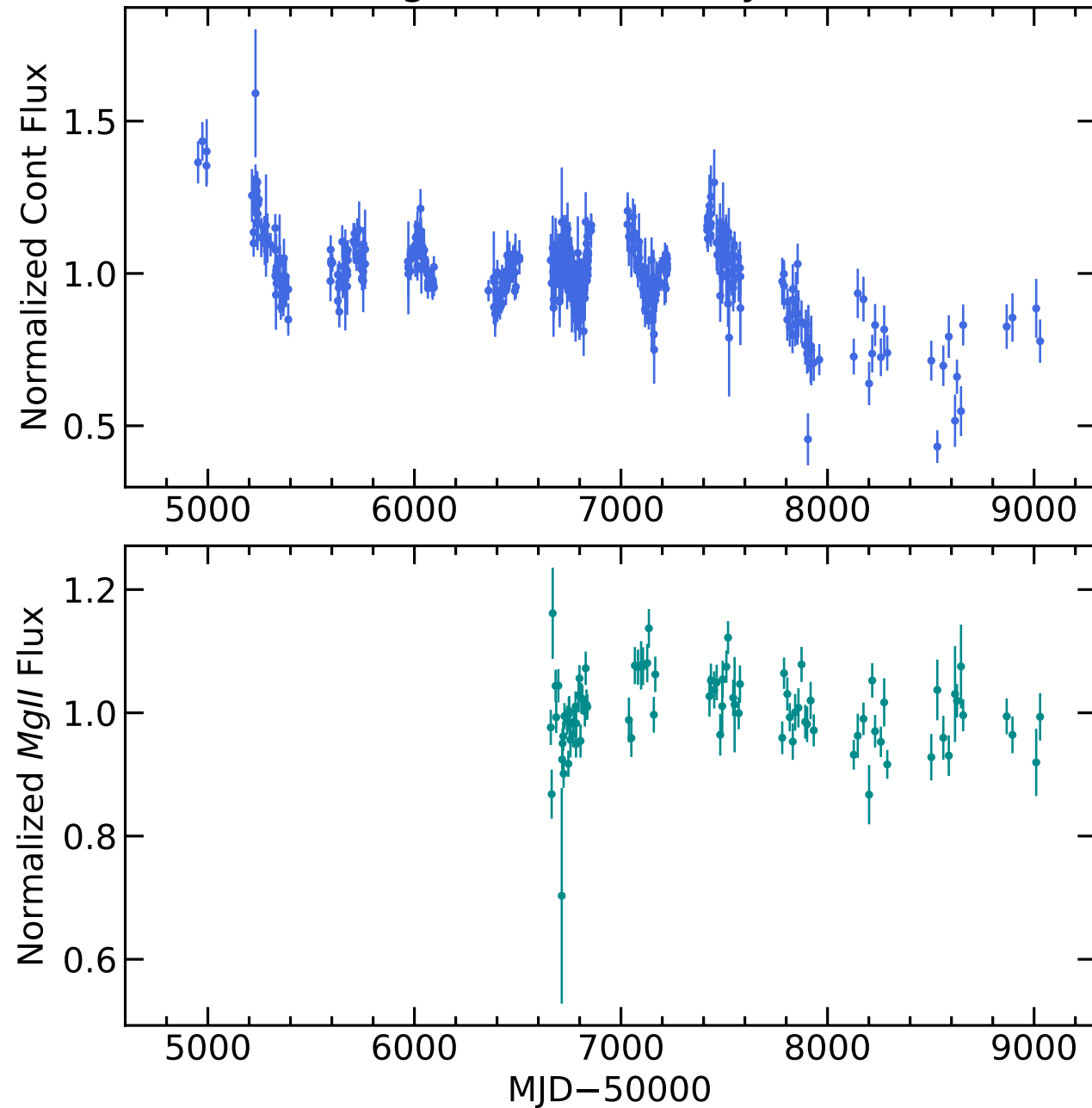
RM406 Light Curves (w/ PyROA model)
