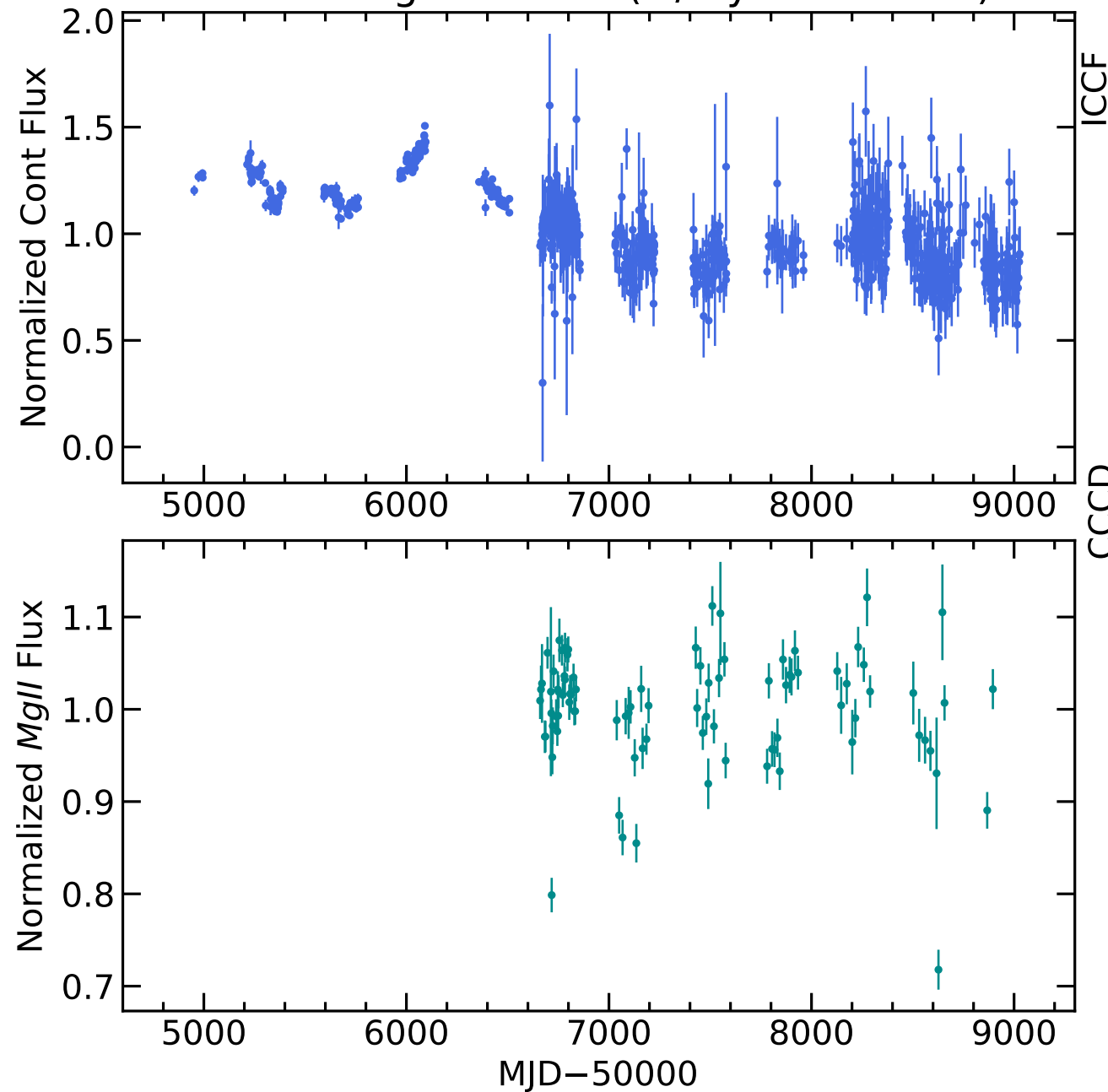
RM407 Light Curves (w/ PyROA model)
