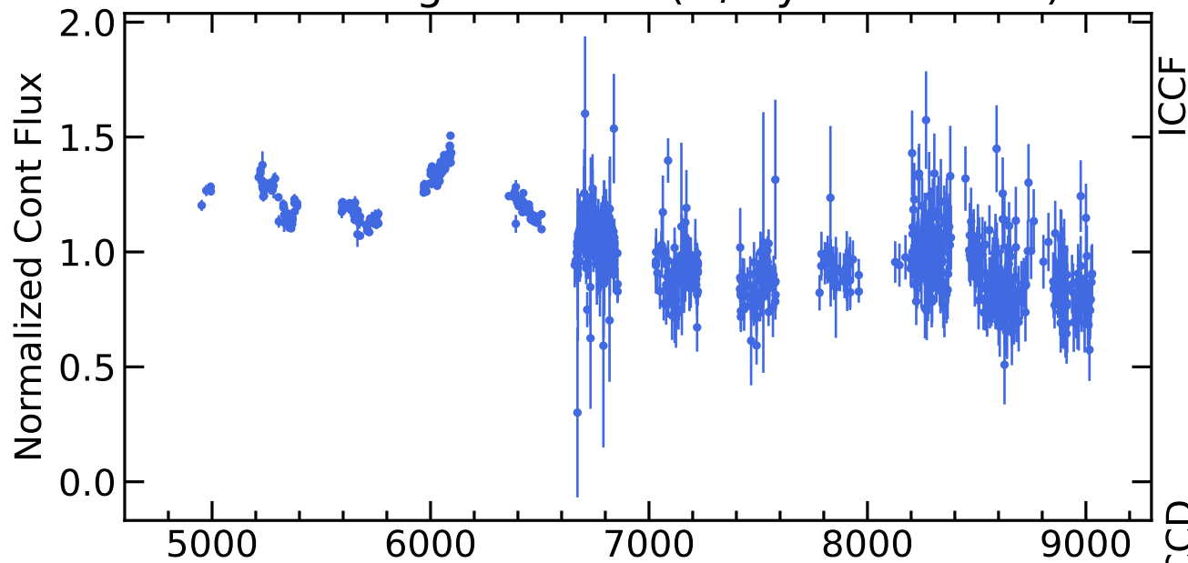
RM407 Light Curves (w/ PyROA model)
